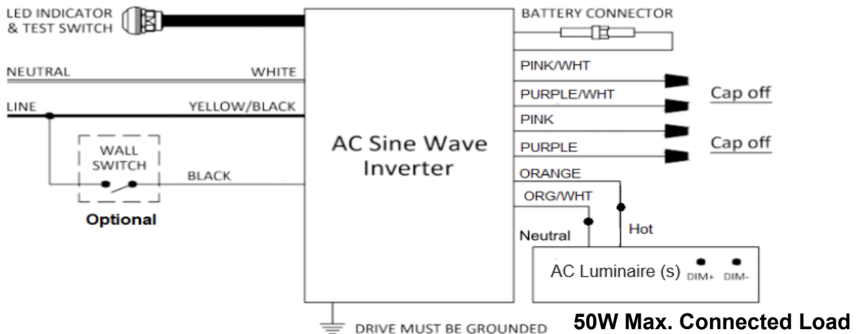
Figure B. Wiring Diagram without 0-10V Dimmer
