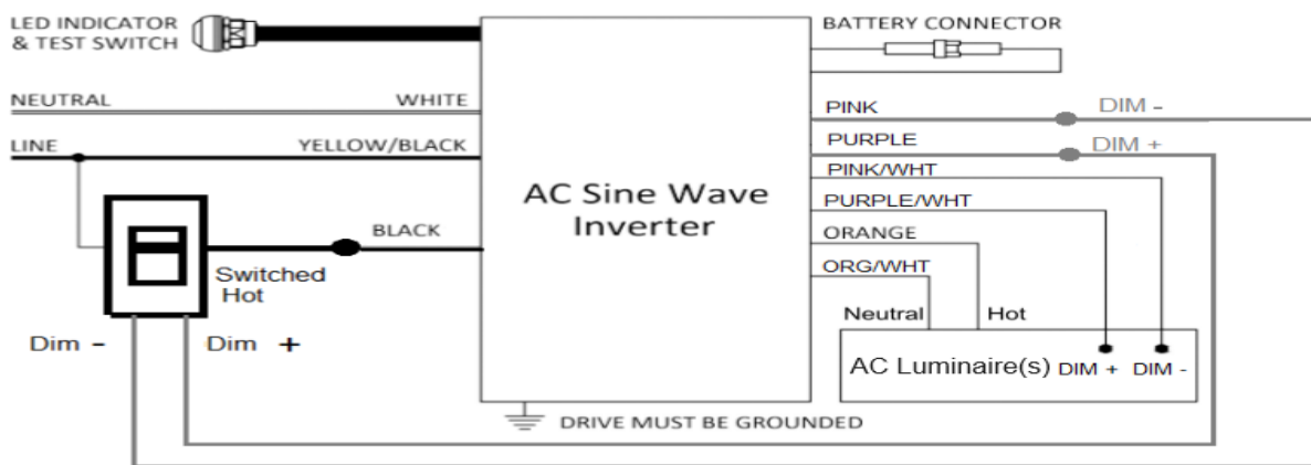
Figure A. Wiring Diagram with 0-10V Dimmer
